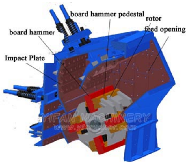
Chart of PF Impact Crusher
